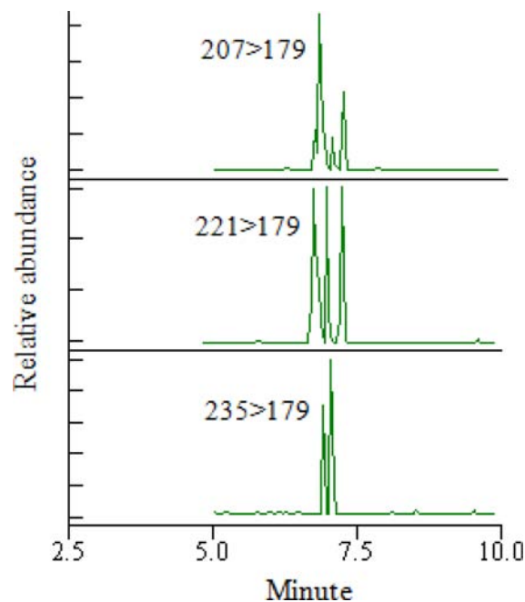
Figure 2. Typical MS-MS chromatograms for 4-NP spiked into tomato samples under optimized conditions. 4-NP was spiked at 50 \mu\text{g kg}^{-1} . Precursor m/z fragments were 207, 221, and 235. Product/quantification m/z is 179 for each precursor.
